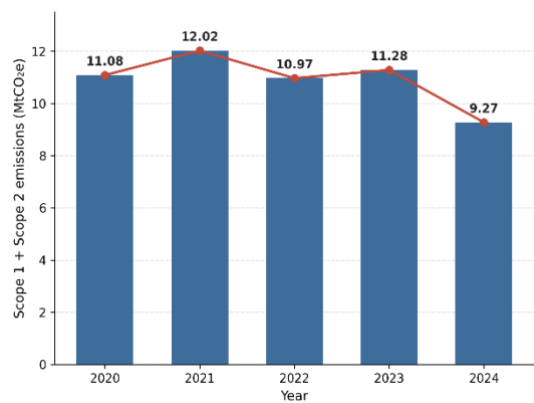
Figure 1. Annual combined Scope 1 and Scope 2 greenhouse-gas emissions of PT KPI, 2020–2024 (million tonnes CO 2 -equivalent). Emissions rose to a peak of 12.02 MtCO 2 e in 2021, declined in 2022, increased again in 2023, and fell to 9.27 MtCO 2 e in 2024—a net reduction of 16.3% relative to the 2020 baseline of 11.08 MtCO 2 e.
