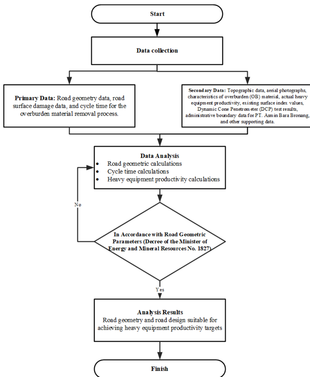
Figure 1. Research workflow
